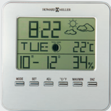
WEATHER VIEW
